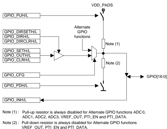
Figure 5. GPIO Control Logic
