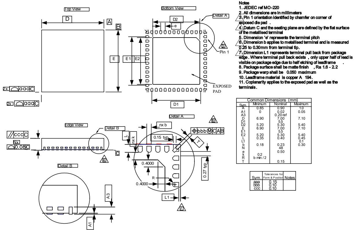
Figure 17. Package Drawing
